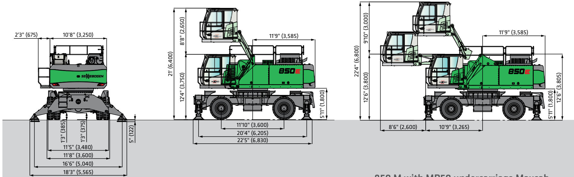
850 M with MP50 undercarriage and Maxcab E270 cab with hydraulic elevation feature
